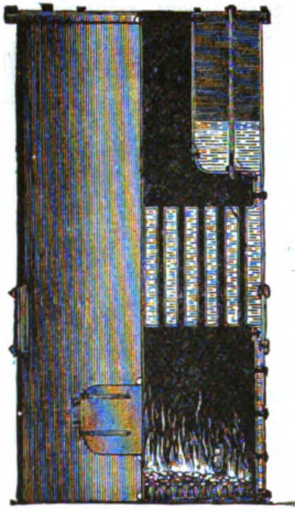
FIG. 23.—THE UPRIGHT BOILER.
